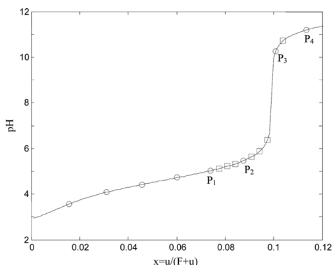
Fig. 3. A titration curve and the proposed dosing sequence (simulation). Sample solution: HCl (0.001 mol/L), acetic acid (0.008 mol/L, K_a = 1.8 \times 10^{-5} ), and benzoic acid (0.002 mol/L, K_a = 6.28 \times 10^{-5} ), titrating reagent: NaOH (0.1 mol/L).
